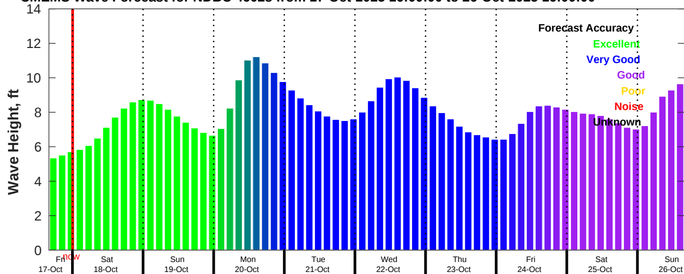
CMEMS Wave Forecast for NDBC 46028 from 17-Oct-2025 16:00:00 to 26-Oct-2025 16:00:00
