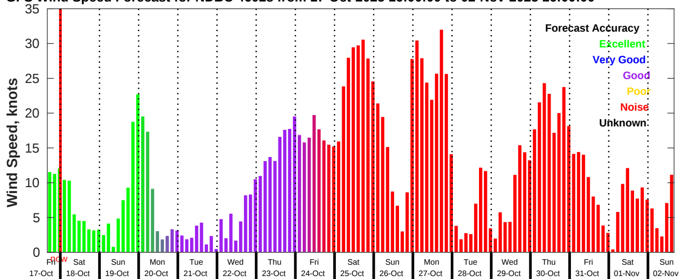
GFS Wind Speed Forecast for NDBC 46028 from 17-Oct-2025 16:00:00 to 02-Nov-2025 16:00:00
