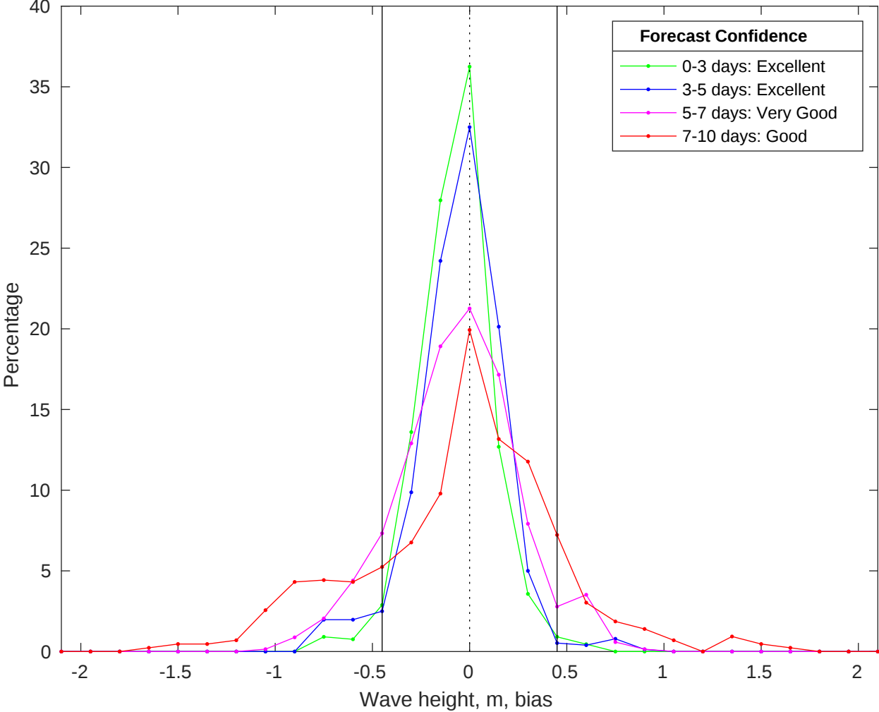
NDBC 46054 vs CMEMS Waves Bias Histogram: 18-Oct-2025
