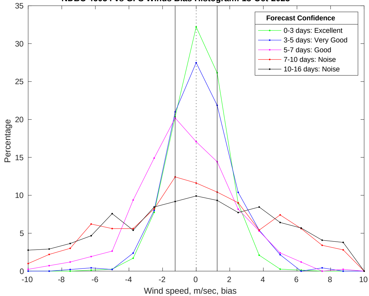
NDBC 46054 vs GFS Winds Bias Histogram: 18-Oct-2025
