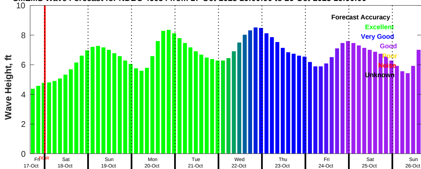
CMEMS Wave Forecast for NDBC 46054 from 17-Oct-2025 16:00:00 to 26-Oct-2025 16:00:00
