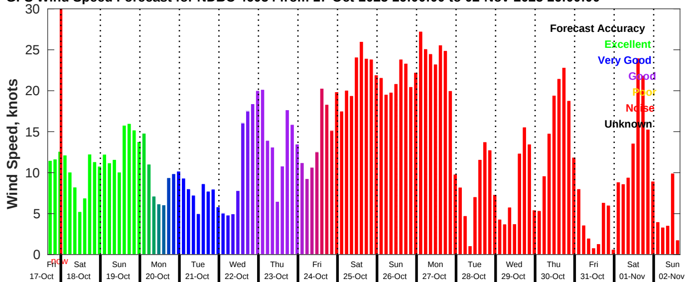
GFS Wind Speed Forecast for NDBC 46054 from 17-Oct-2025 16:00:00 to 02-Nov-2025 16:00:00
