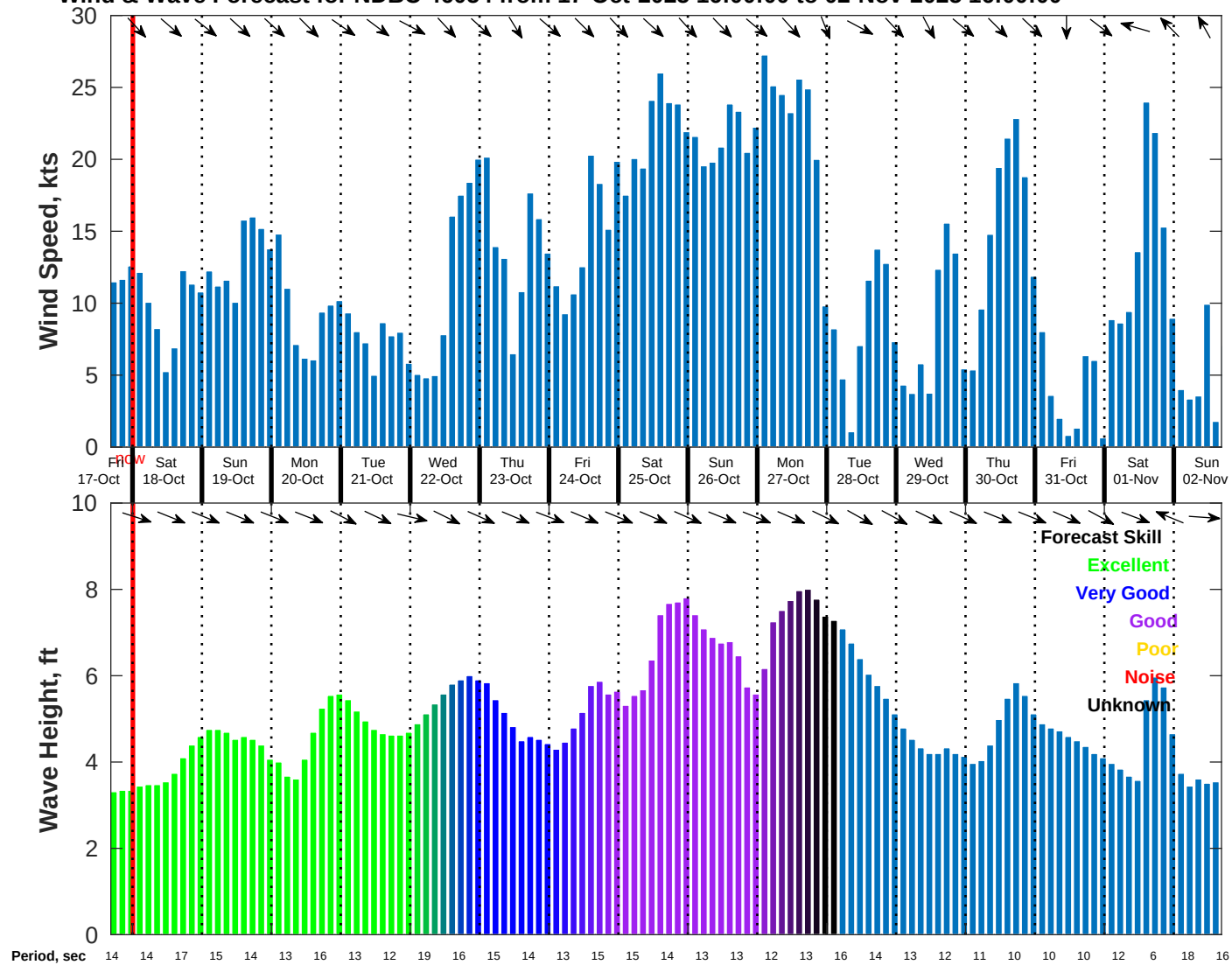
Wind & Wave Forecast for NDBC 46054 from 17-Oct-2025 16:00:00 to 02-Nov-2025 16:00:00
