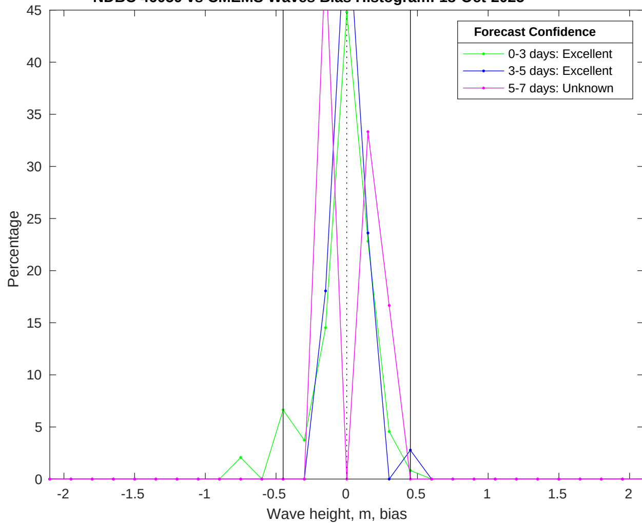
NDBC 46059 vs CMEMS Waves Bias Histogram: 18-Oct-2025
