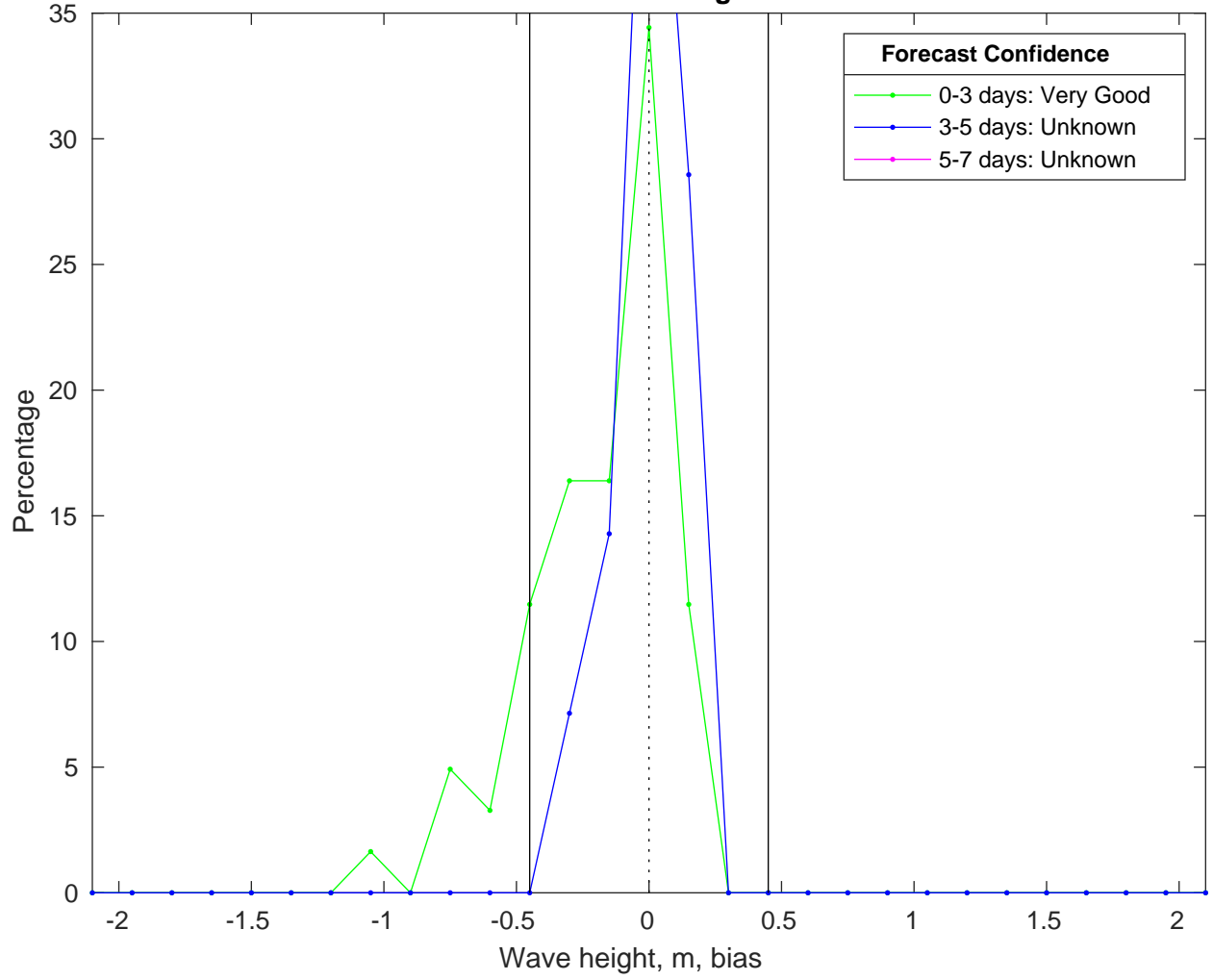
NDBC 46059 vs GFS Waves Bias Histogram: 18-Oct-2025
