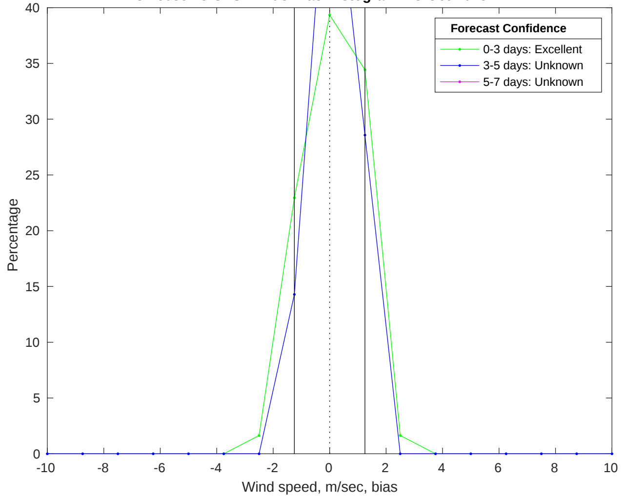
NDBC 46059 vs GFS Winds Bias Histogram: 18-Oct-2025
