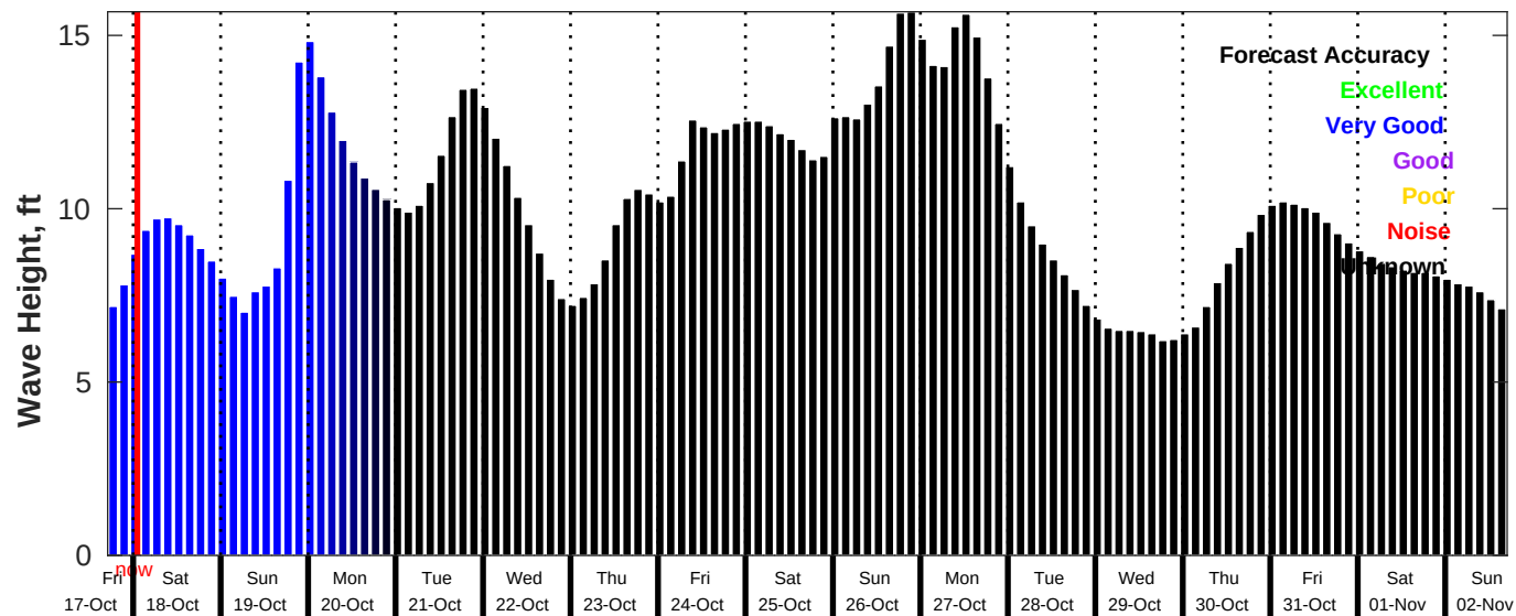
GFS Wave Forecast for NDBC 46059 from 17-Oct-2025 17:00:00 to 02-Nov-2025 17:00:00
