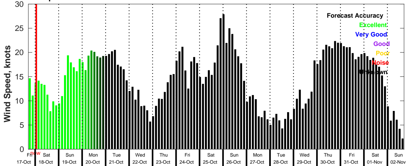
GFS Wind Speed Forecast for NDBC 46059 from 17-Oct-2025 17:00:00 to 02-Nov-2025 17:00:00
