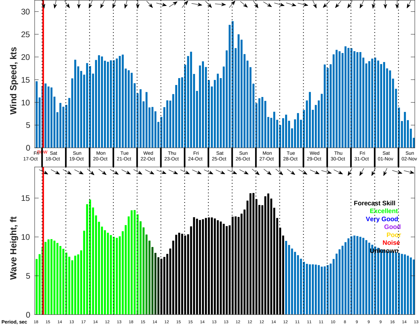
Wind & Wave Forecast for NDBC 46059 from 17-Oct-2025 17:00:00 to 02-Nov-2025 17:00:00
