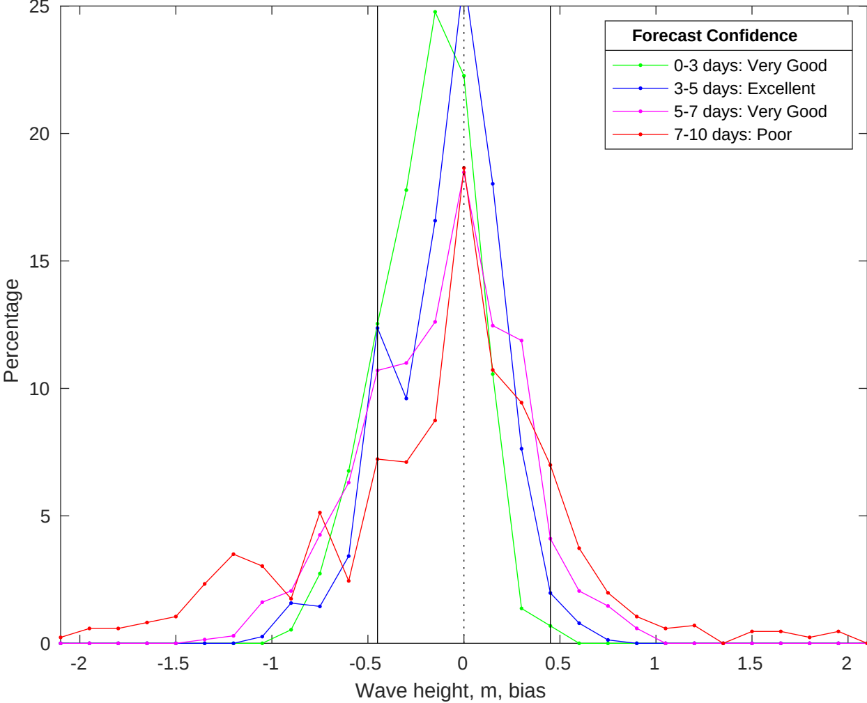
NDBC 46069 vs CMEMS Waves Bias Histogram: 18-Oct-2025
