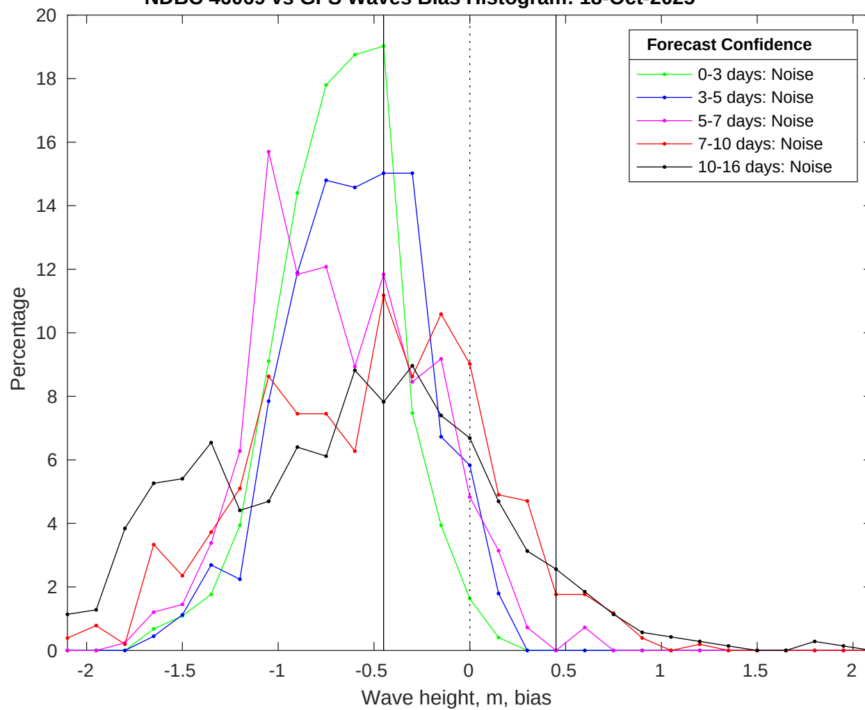
NDBC 46069 vs GFS Waves Bias Histogram: 18-Oct-2025
