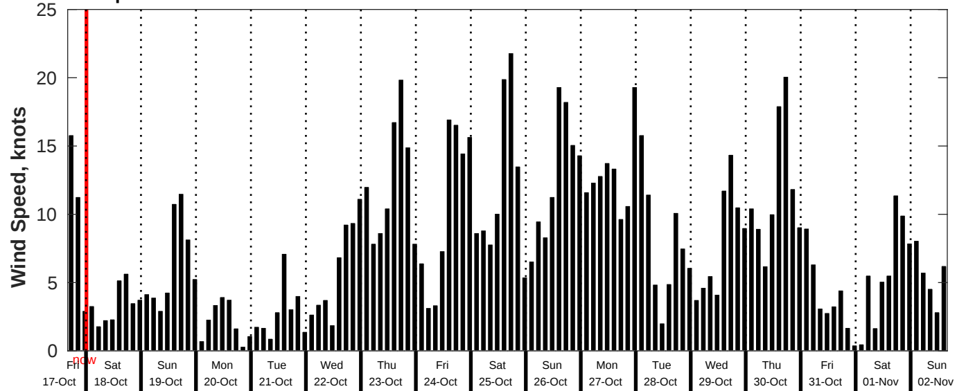
GFS Wind Speed Forecast for NDBC 46215 from 17-Oct-2025 16:00:00 to 02-Nov-2025 16:00:00
