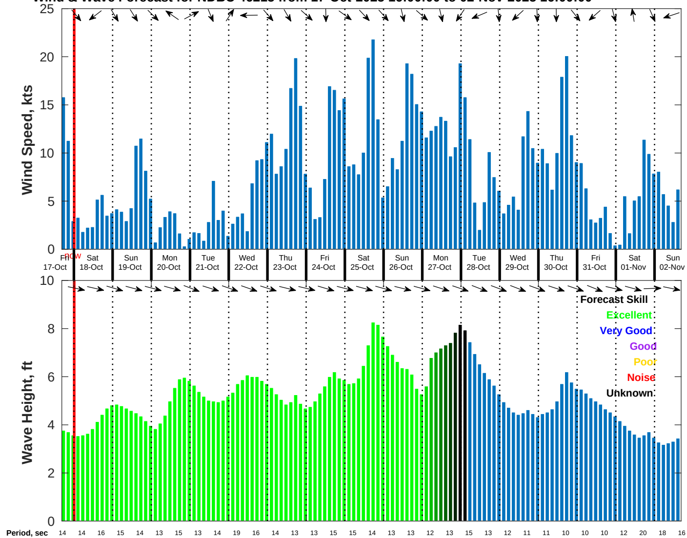
Wind & Wave Forecast for NDBC 46215 from 17-Oct-2025 16:00:00 to 02-Nov-2025 16:00:00
