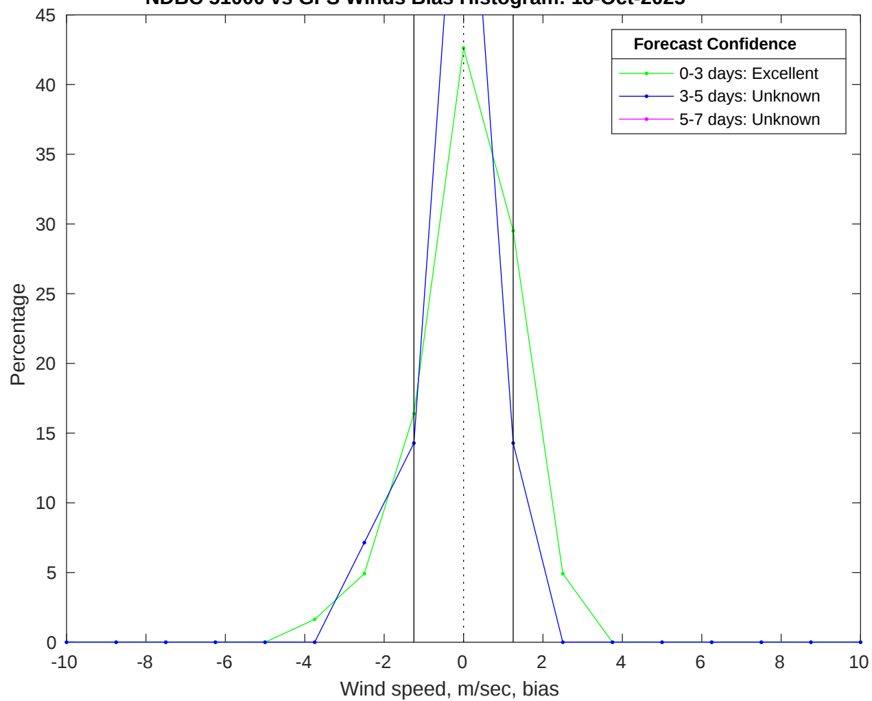
NDBC 51000 vs GFS Winds Bias Histogram: 18-Oct-2025
