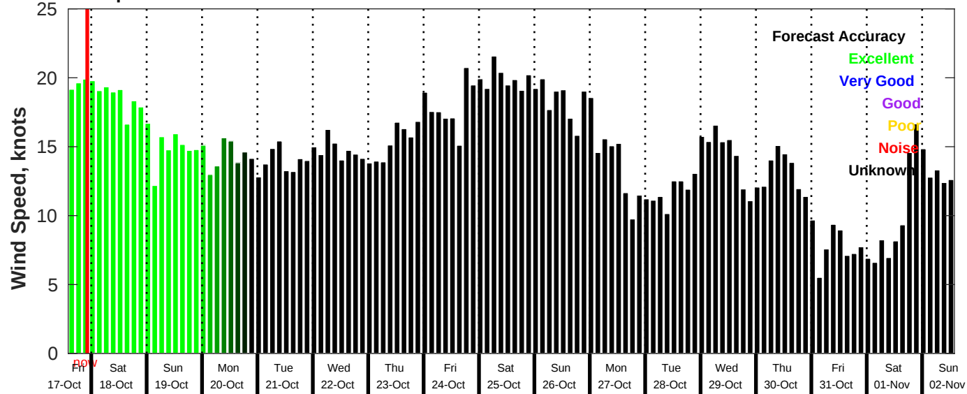
GFS Wind Speed Forecast for NDBC 51000 from 17-Oct-2025 14:00:00 to 02-Nov-2025 14:00:00
