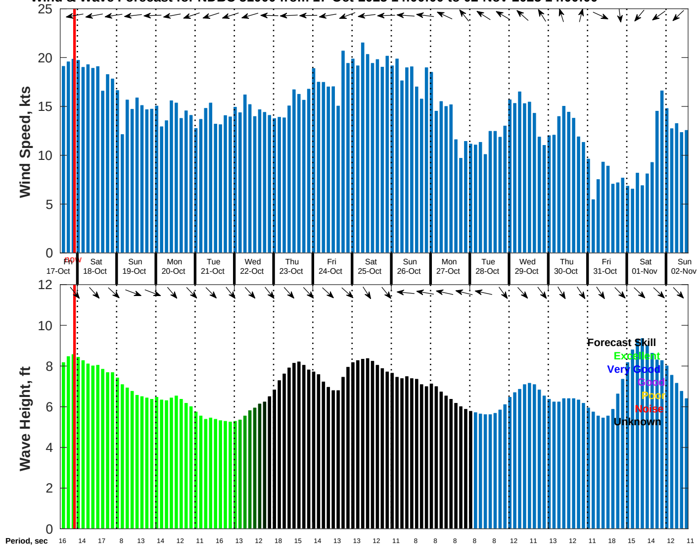
Wind & Wave Forecast for NDBC 51000 from 17-Oct-2025 14:00:00 to 02-Nov-2025 14:00:00
