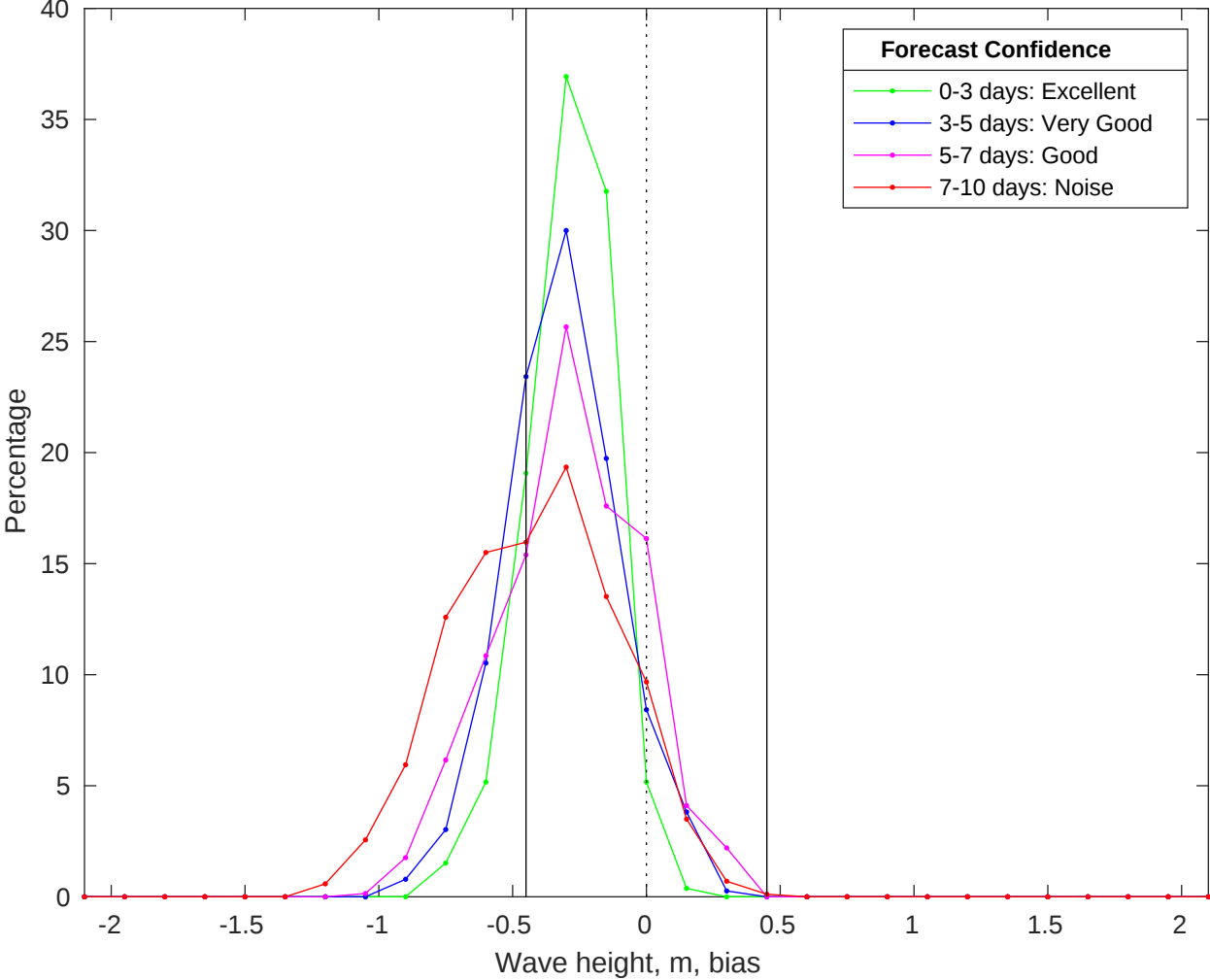
NDBC 51209 vs CMEMS Waves Bias Histogram: 18-Oct-2025
