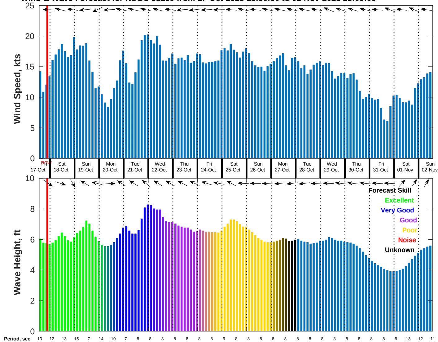
Wind & Wave Forecast for NDBC 51209 from 17-Oct-2025 13:00:00 to 02-Nov-2025 13:00:00
