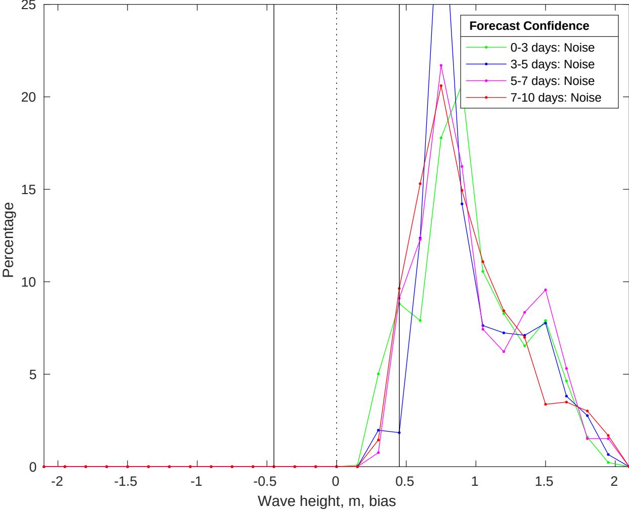
NDBC 51211 vs CMEMS Waves Bias Histogram: 18-Oct-2025
