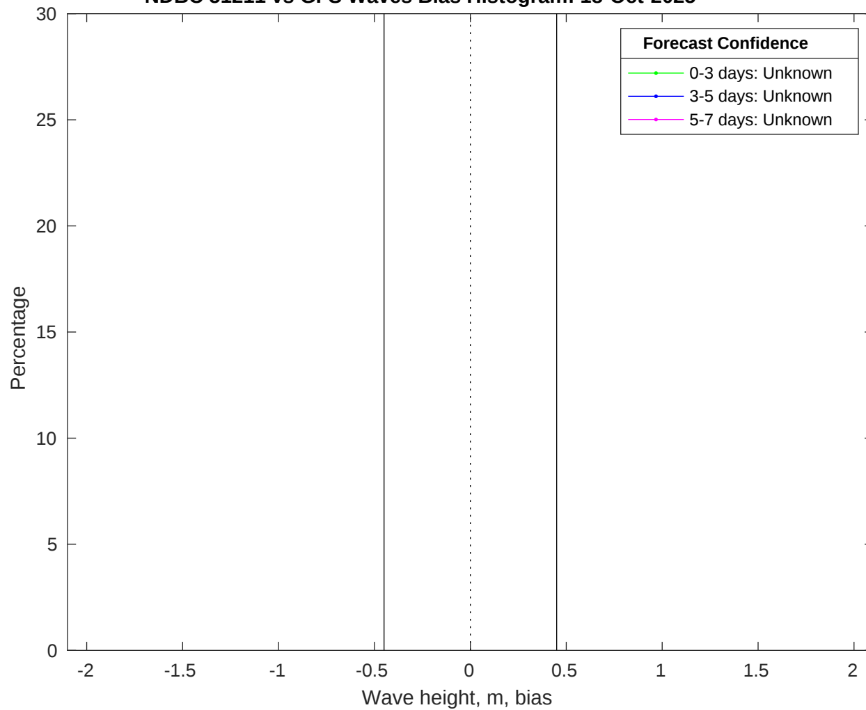
NDBC 51211 vs GFS Waves Bias Histogram: 18-Oct-2025
