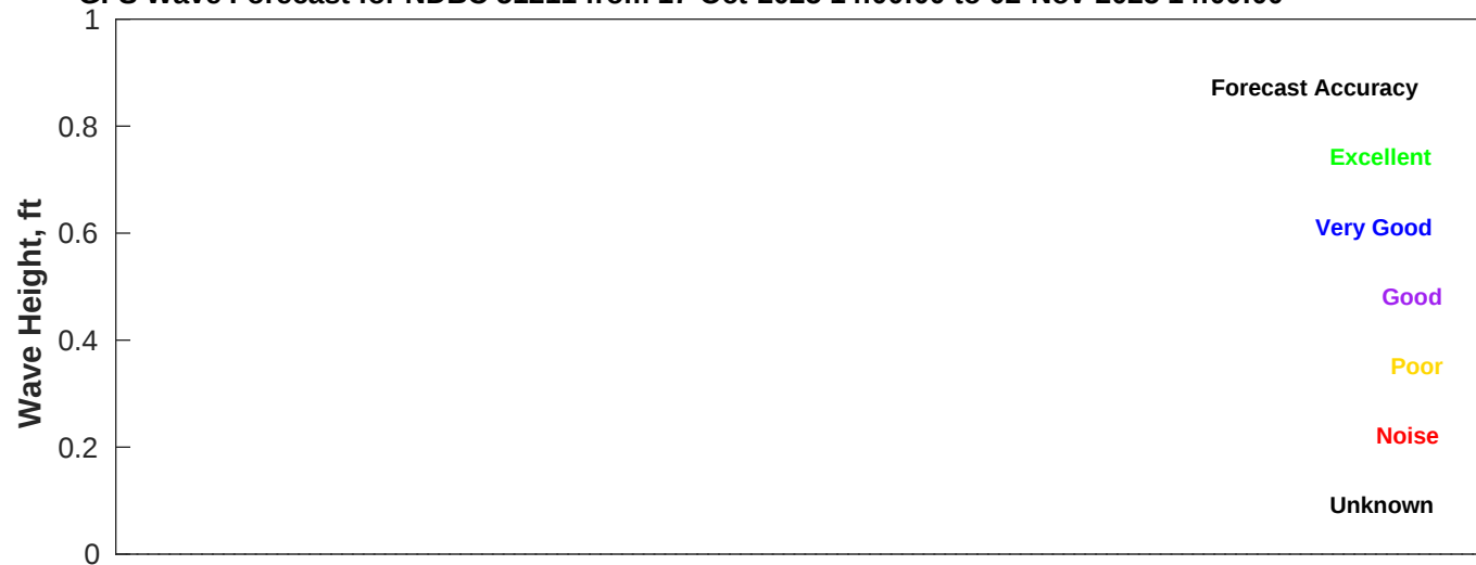
GFS Wave Forecast for NDBC 51211 from 17-Oct-2025 14:00:00 to 02-Nov-2025 14:00:00
