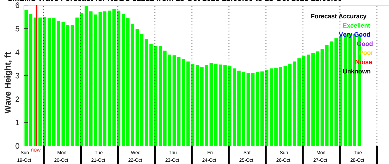
CMEMS Wave Forecast for NDBC 52211 from 18-Oct-2025 11:00:00 to 28-Oct-2025 11:00:00
