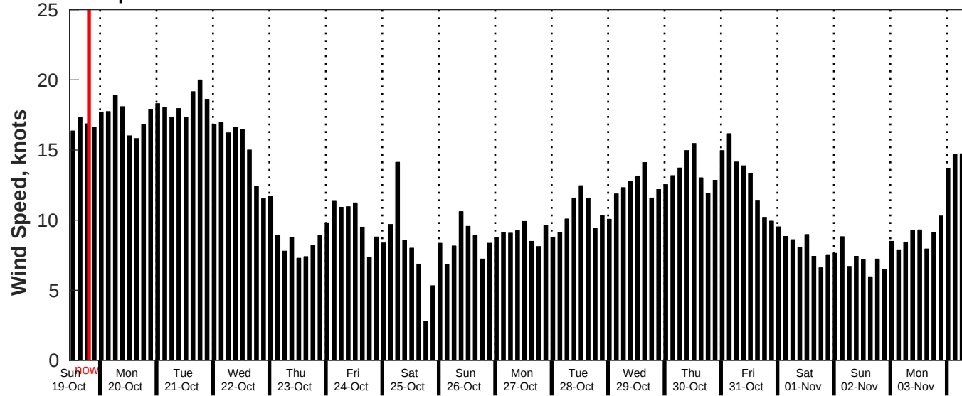
GFS Wind Speed Forecast for NDBC 52211 from 18-Oct-2025 11:00:00 to 03-Nov-2025 11:00:00
