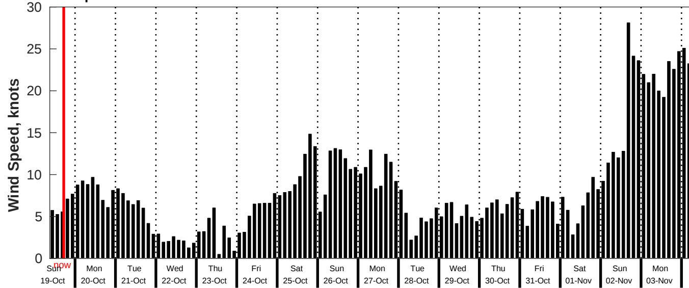
GFS Wind Speed Forecast for NDBC 52212 from 18-Oct-2025 09:00:00 to 03-Nov-2025 09:00:00
