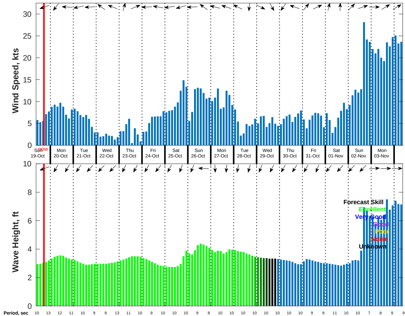
Wind & Wave Forecast for NDBC 52212 from 18-Oct-2025 09:00:00 to 03-Nov-2025 09:00:00
