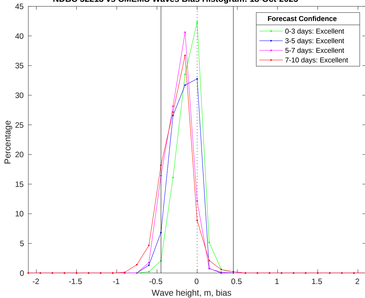
NDBC 52213 vs CMEMS Waves Bias Histogram: 18-Oct-2025
