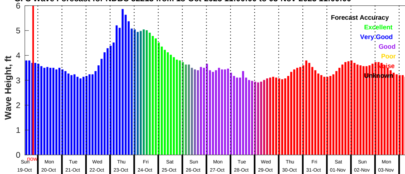
GFS Wave Forecast for NDBC 52213 from 18-Oct-2025 11:00:00 to 03-Nov-2025 11:00:00
