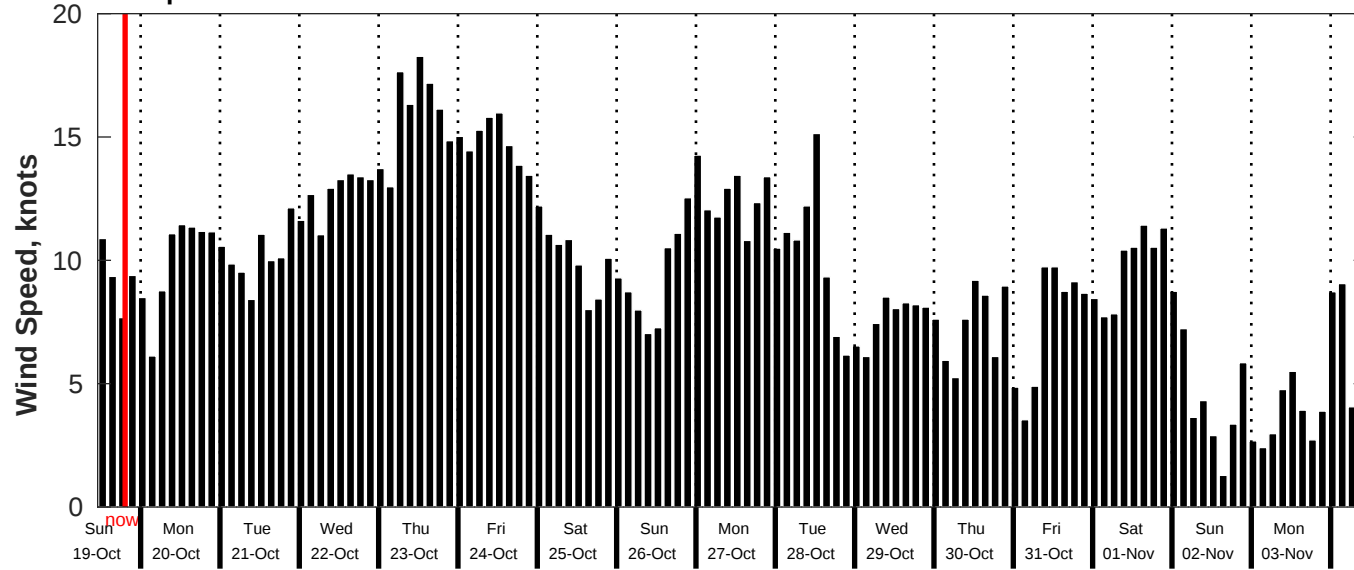
GFS Wind Speed Forecast for NDBC 52213 from 18-Oct-2025 11:00:00 to 03-Nov-2025 11:00:00
