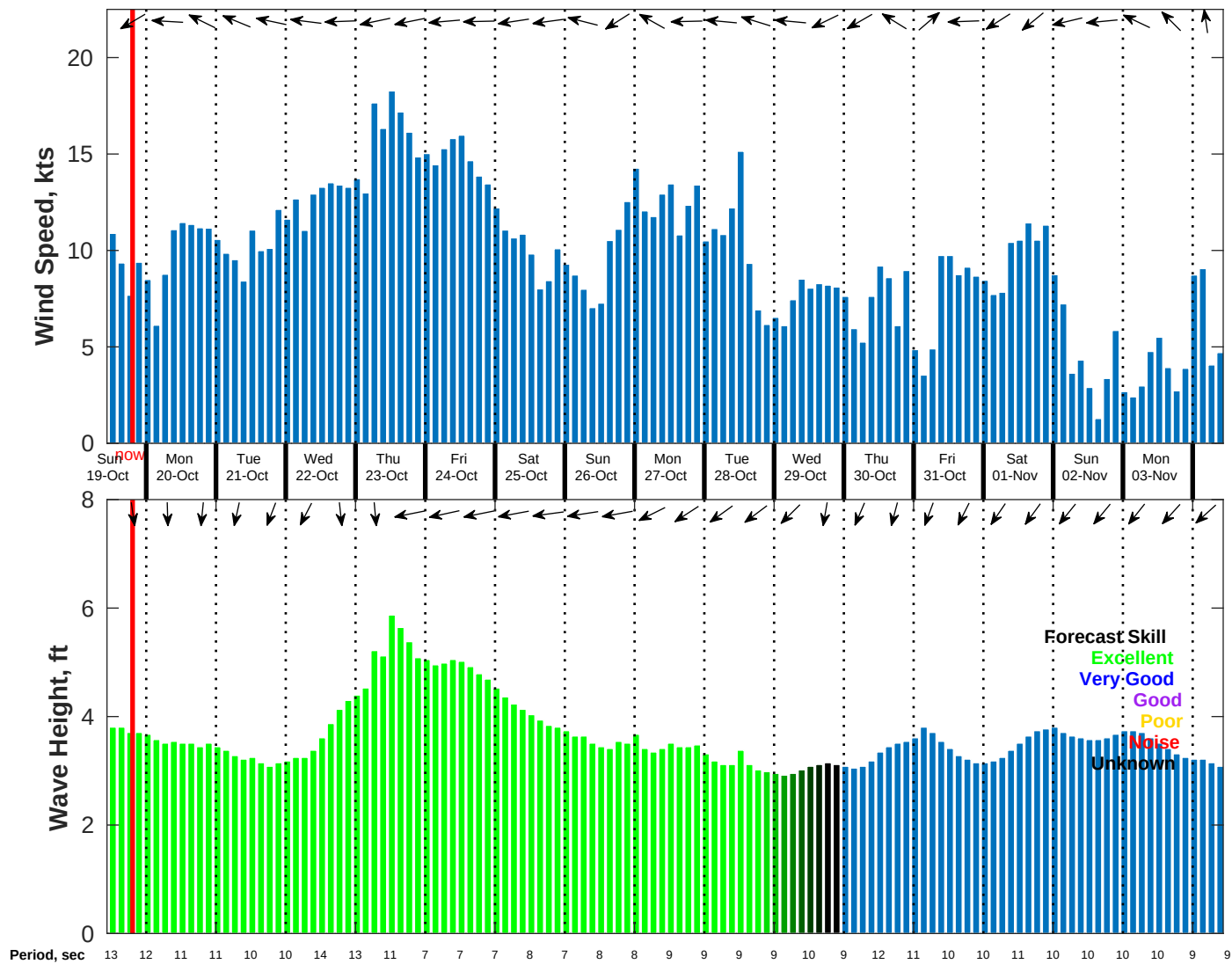
Wind & Wave Forecast for NDBC 52213 from 18-Oct-2025 11:00:00 to 03-Nov-2025 11:00:00
