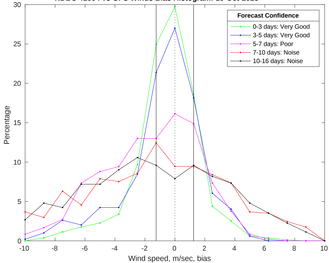
NDBC 41004 vs GFS Winds Bias Histogram: 19-Oct-2025
