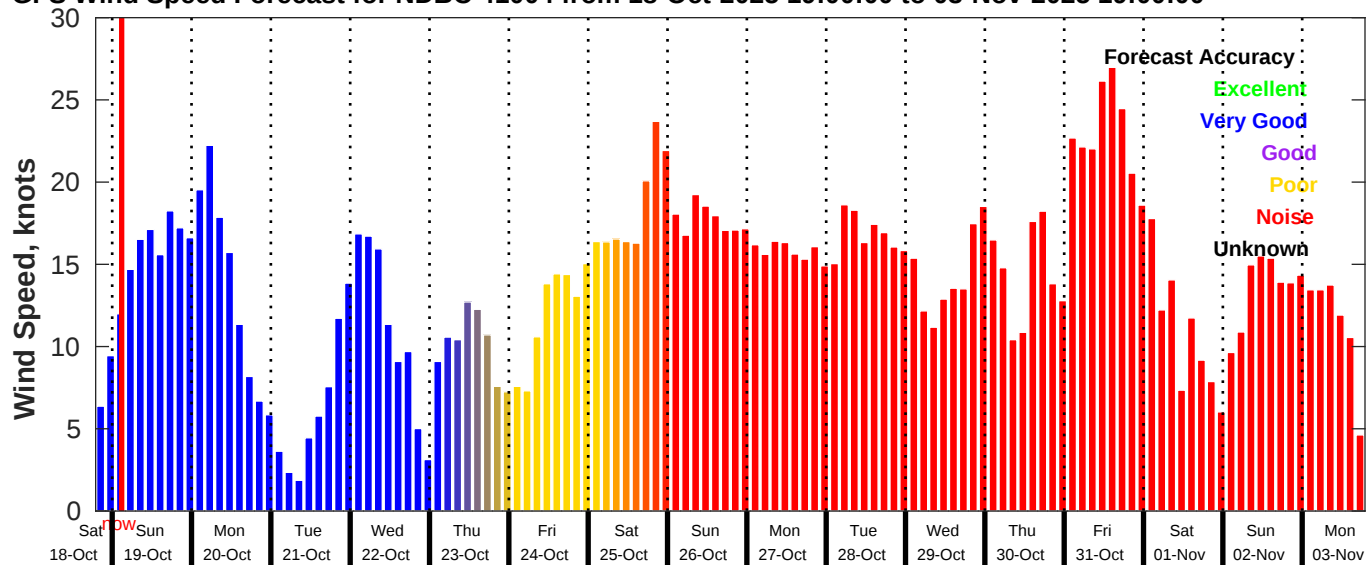
GFS Wind Speed Forecast for NDBC 41004 from 18-Oct-2025 19:00:00 to 03-Nov-2025 19:00:00
