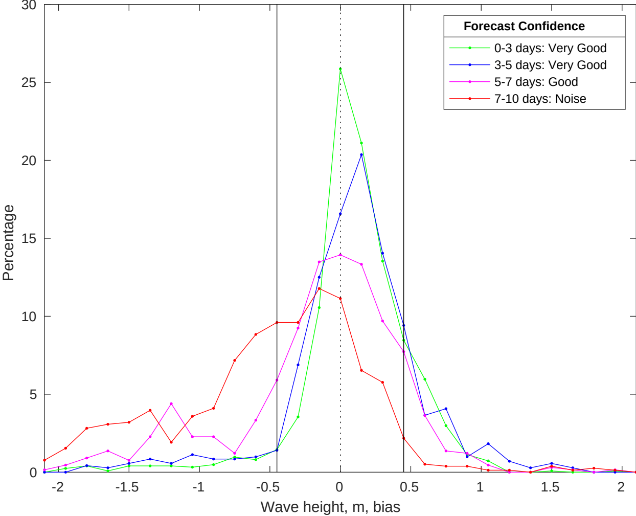
NDBC 41013 vs CMEMS Waves Bias Histogram: 19-Oct-2025
