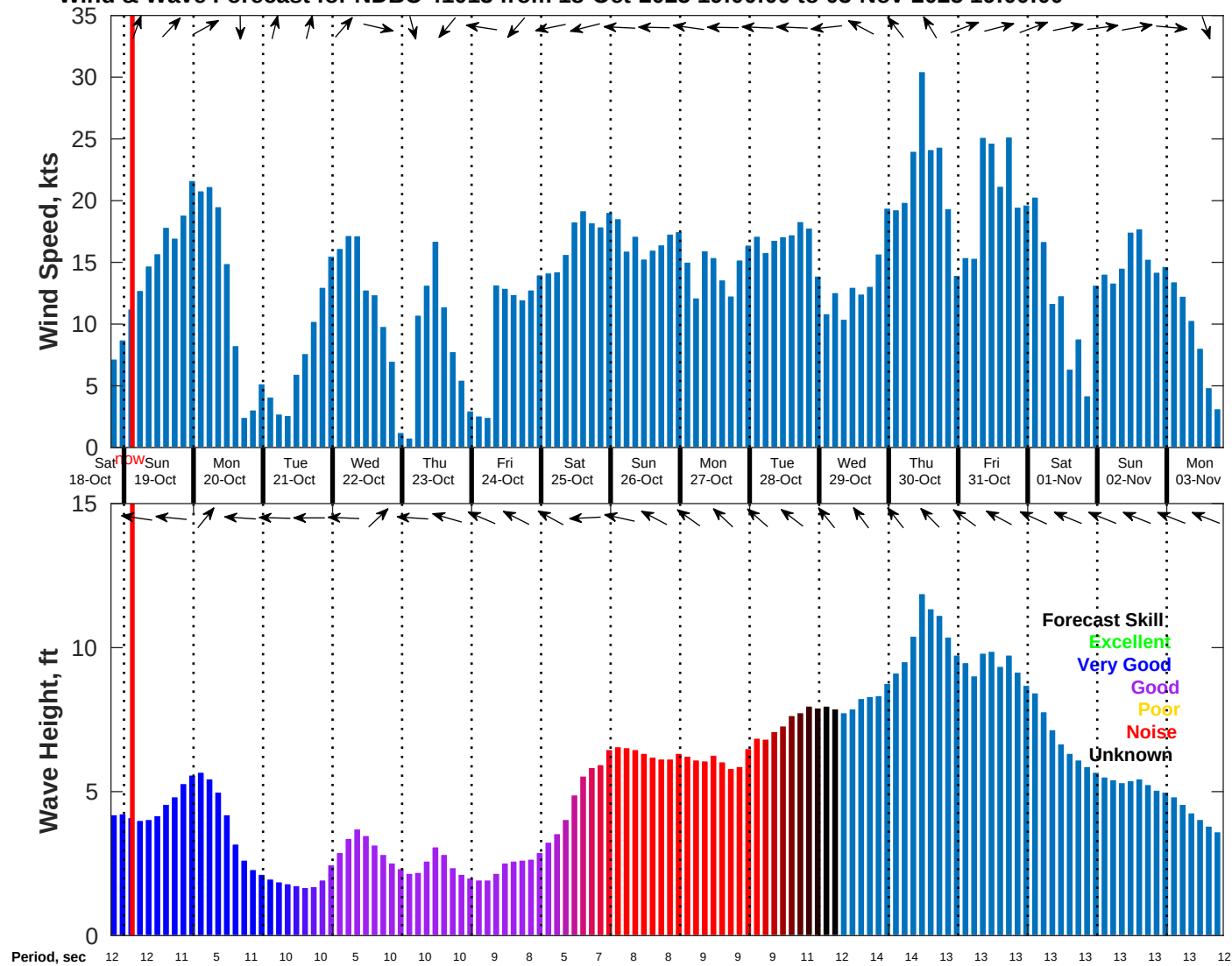
Wind & Wave Forecast for NDBC 41013 from 18-Oct-2025 19:00:00 to 03-Nov-2025 19:00:00
