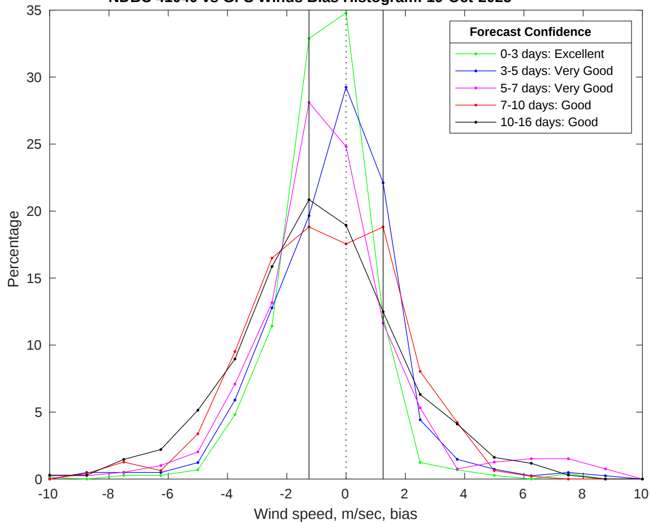
NDBC 41040 vs GFS Winds Bias Histogram: 19-Oct-2025
