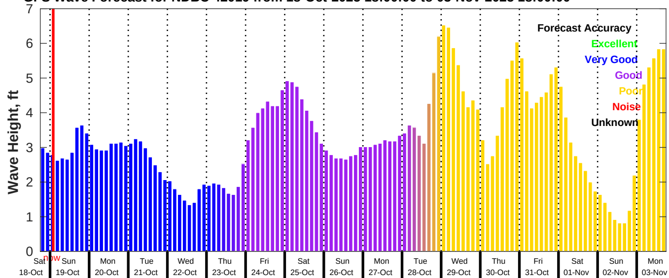
GFS Wave Forecast for NDBC 42019 from 18-Oct-2025 18:00:00 to 03-Nov-2025 18:00:00
