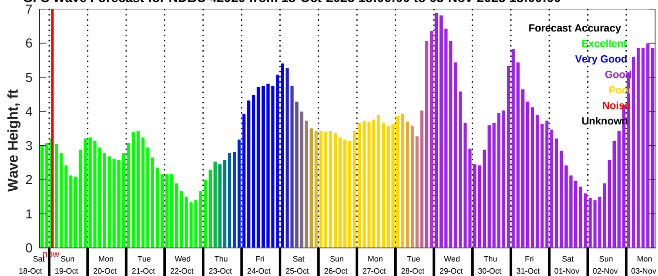
GFS Wave Forecast for NDBC 42020 from 18-Oct-2025 18:00:00 to 03-Nov-2025 18:00:00
