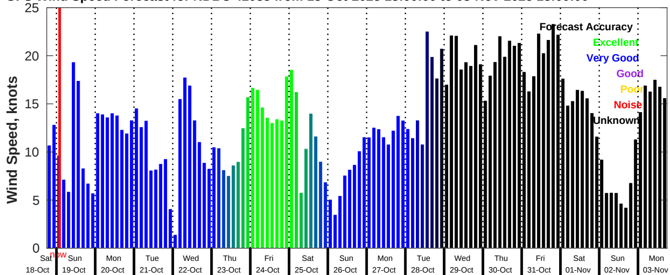
GFS Wind Speed Forecast for NDBC 42035 from 18-Oct-2025 18:00:00 to 03-Nov-2025 18:00:00
