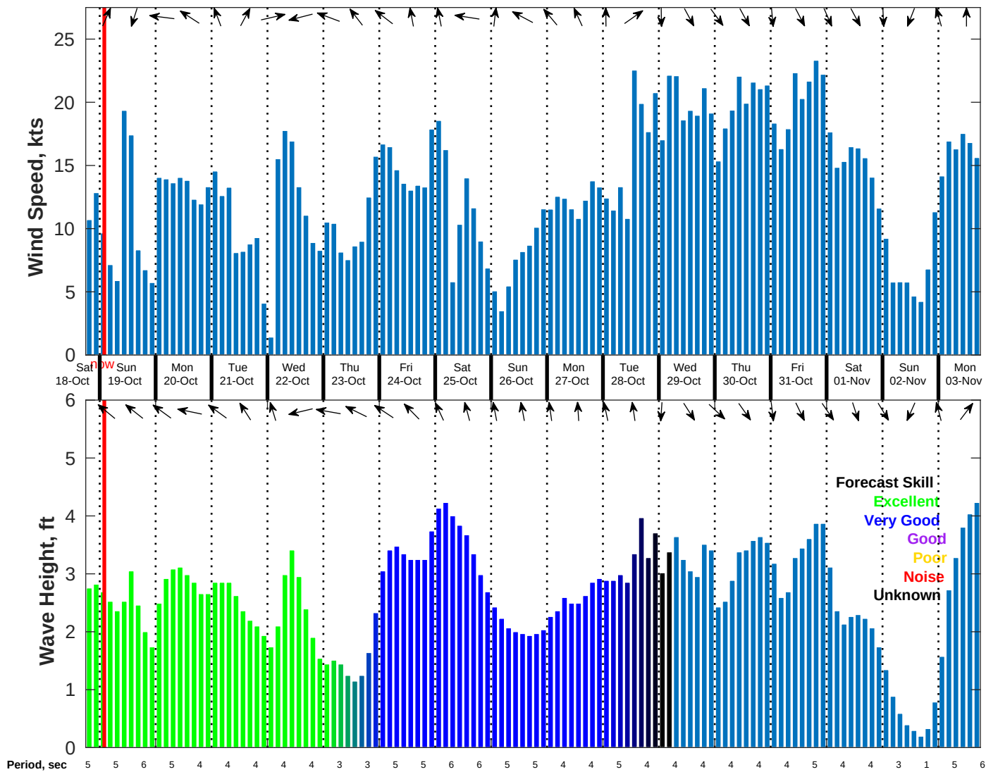
Wind & Wave Forecast for NDBC 42035 from 18-Oct-2025 18:00:00 to 03-Nov-2025 18:00:00
