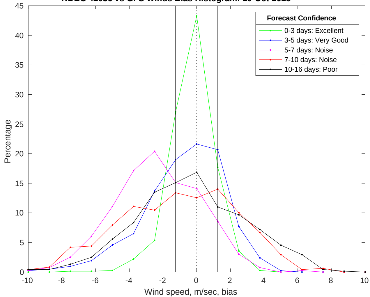
NDBC 42036 vs GFS Winds Bias Histogram: 19-Oct-2025
