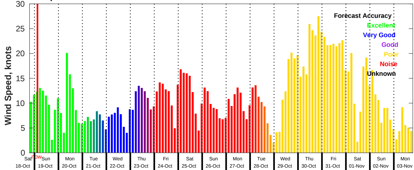
GFS Wind Speed Forecast for NDBC 42036 from 18-Oct-2025 19:00:00 to 03-Nov-2025 19:00:00
