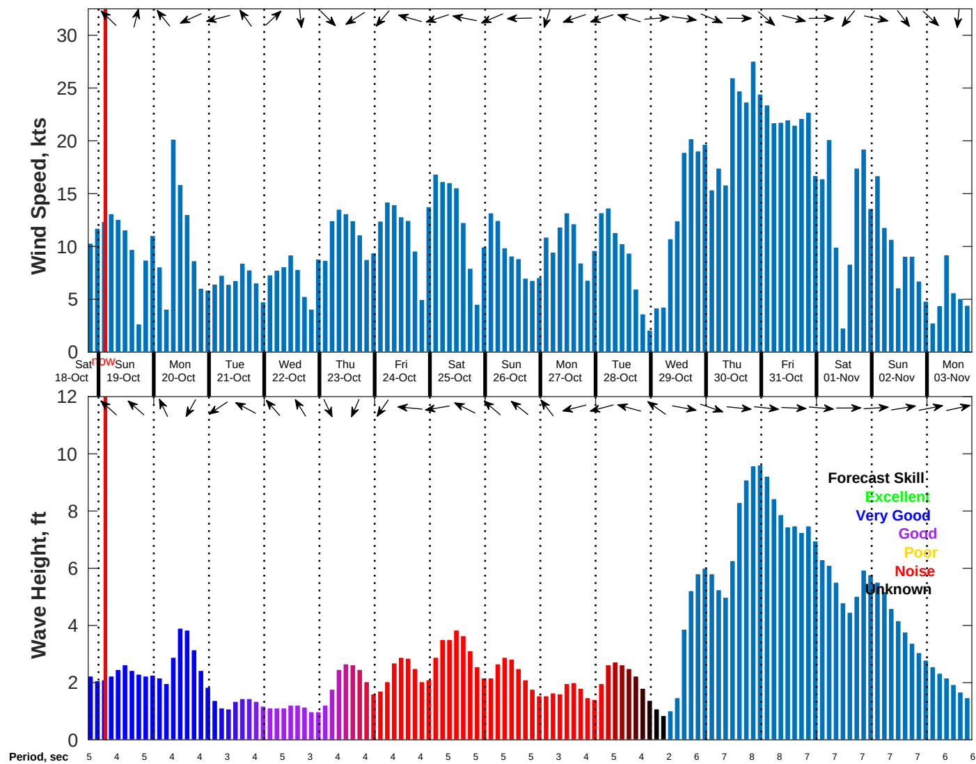
Wind & Wave Forecast for NDBC 42036 from 18-Oct-2025 19:00:00 to 03-Nov-2025 19:00:00
