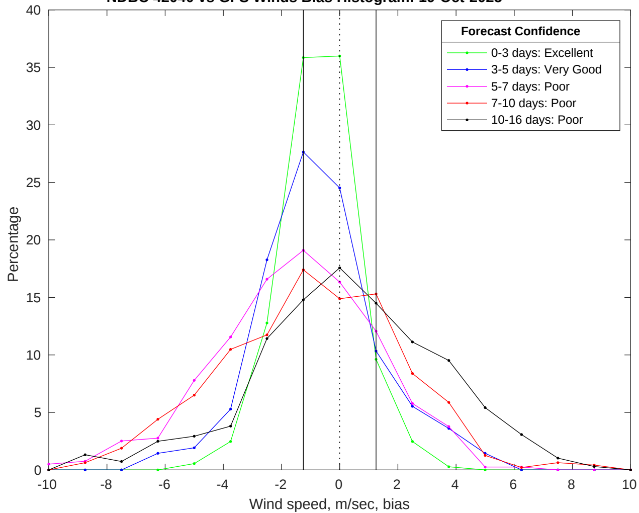
NDBC 42040 vs GFS Winds Bias Histogram: 19-Oct-2025
