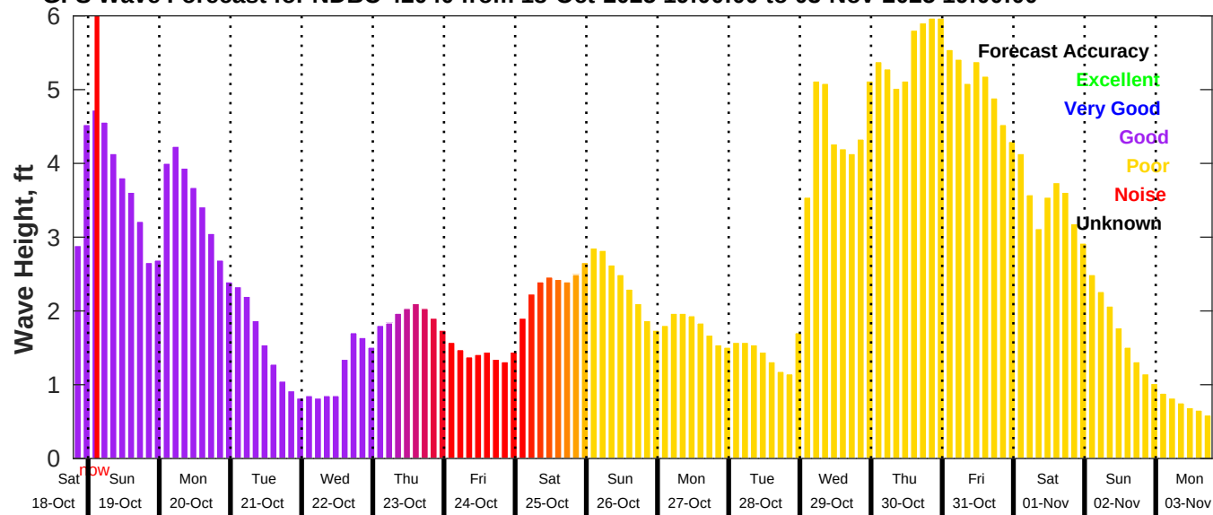
GFS Wave Forecast for NDBC 42040 from 18-Oct-2025 19:00:00 to 03-Nov-2025 19:00:00
