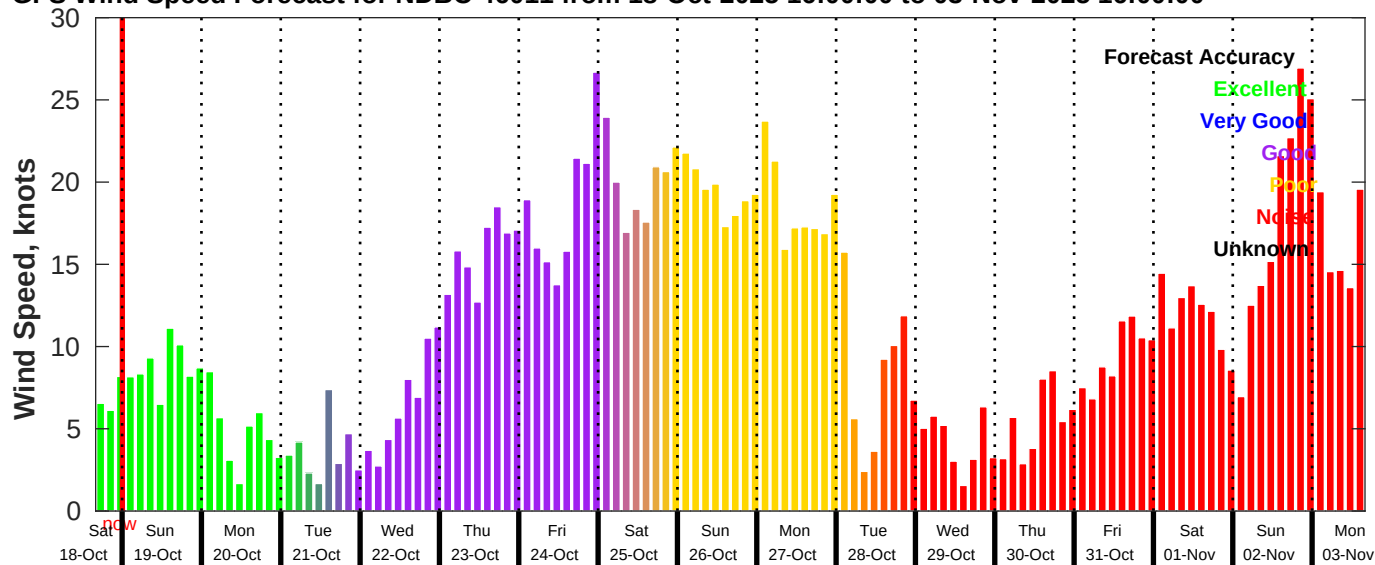
GFS Wind Speed Forecast for NDBC 46011 from 18-Oct-2025 16:00:00 to 03-Nov-2025 16:00:00
