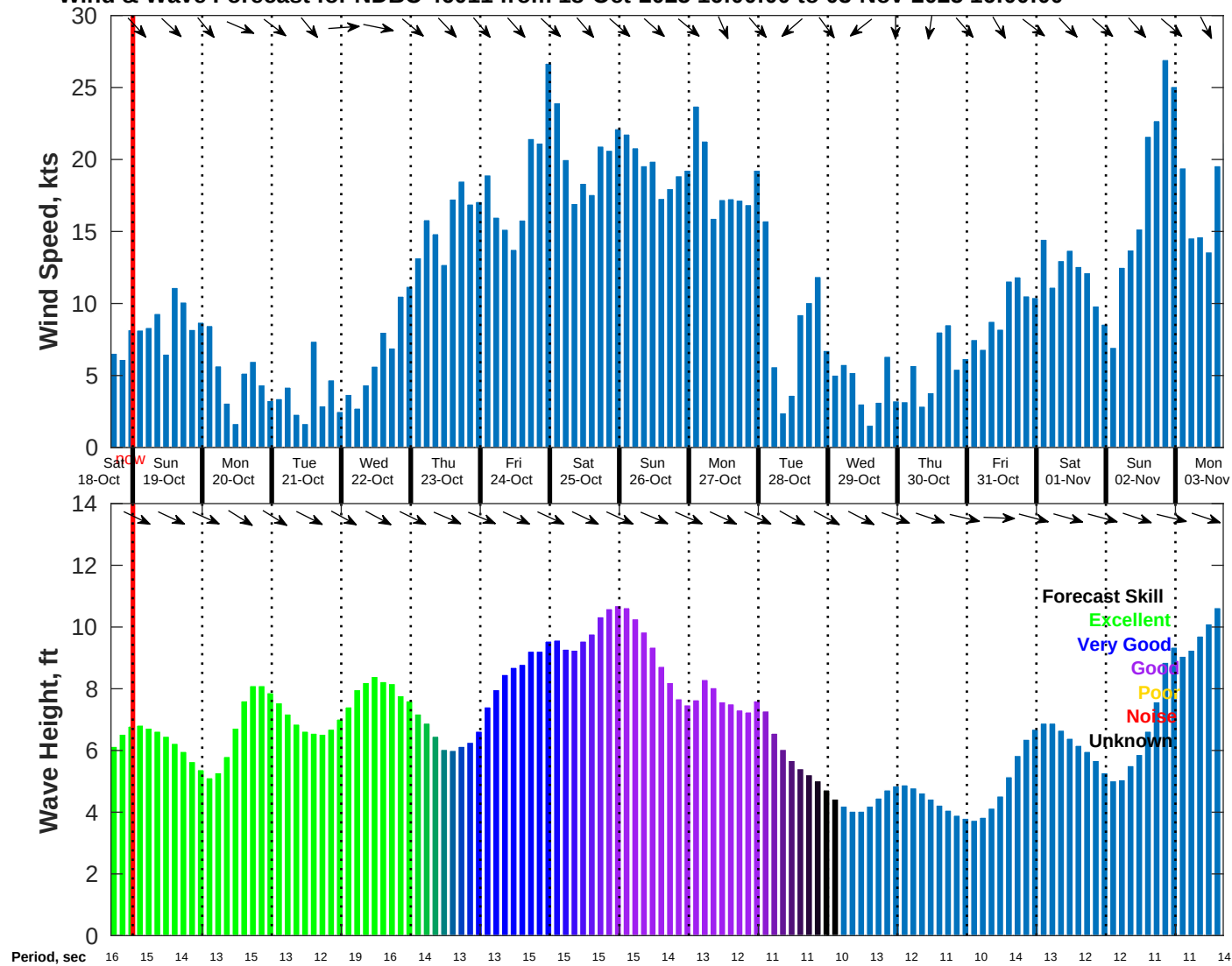
Wind & Wave Forecast for NDBC 46011 from 18-Oct-2025 16:00:00 to 03-Nov-2025 16:00:00
