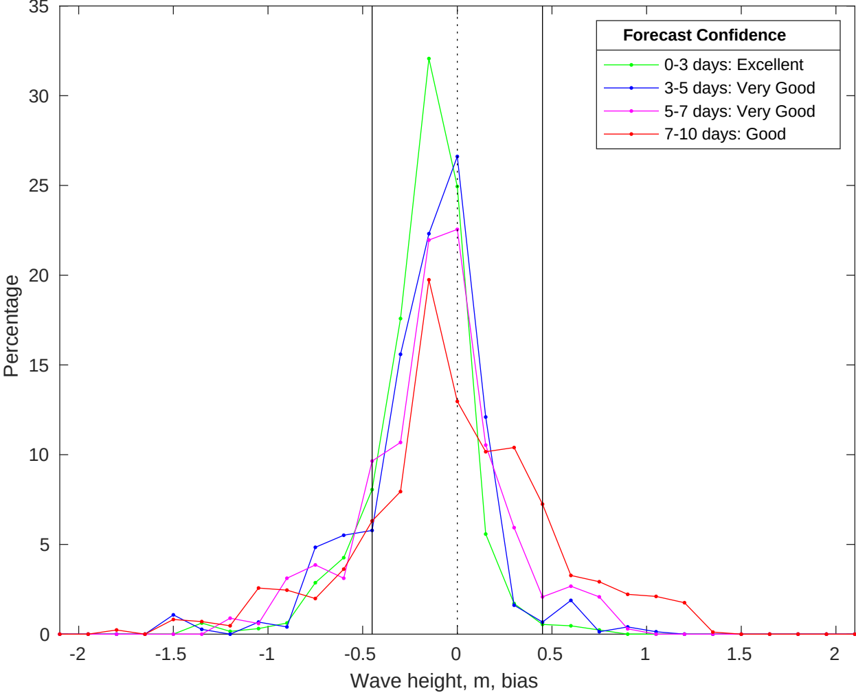
NDBC 46028 vs CMEMS Waves Bias Histogram: 19-Oct-2025
